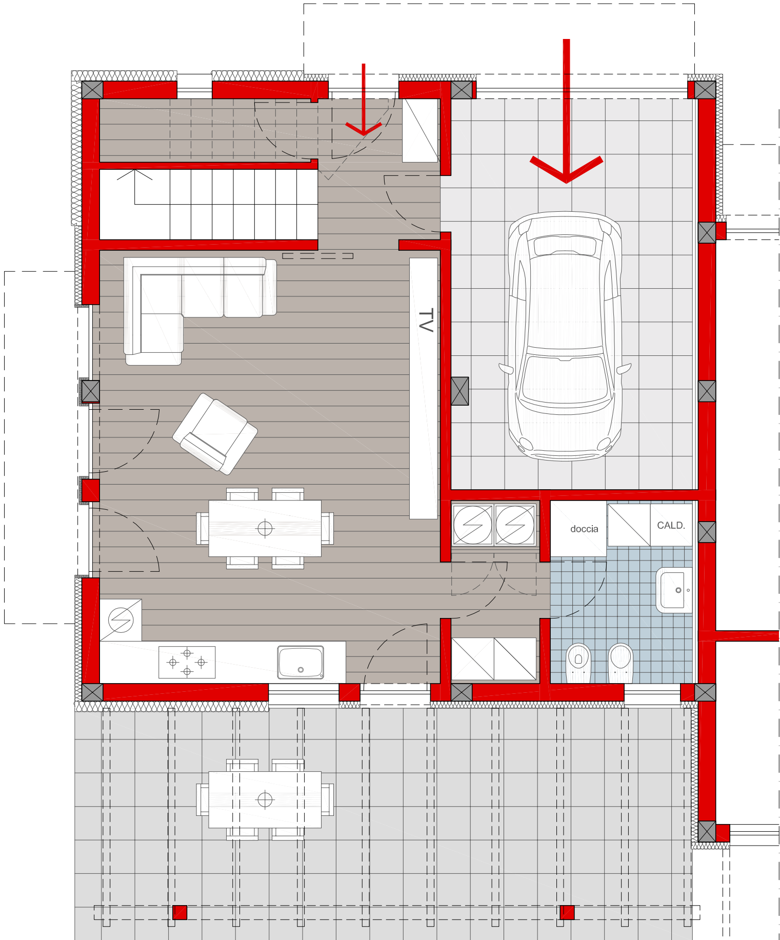
PIANO TERRA
